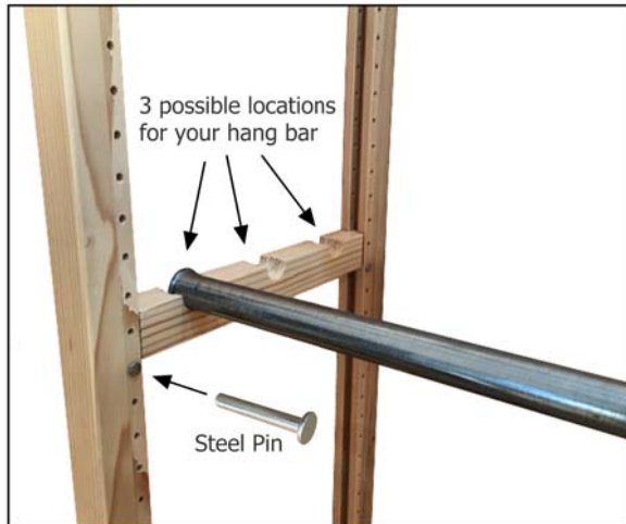
Insert steel pins to desired height of wood support rail
